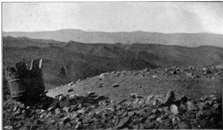
Characteristic View over the mountains in Western Shansi. The archaic range in the distance.
